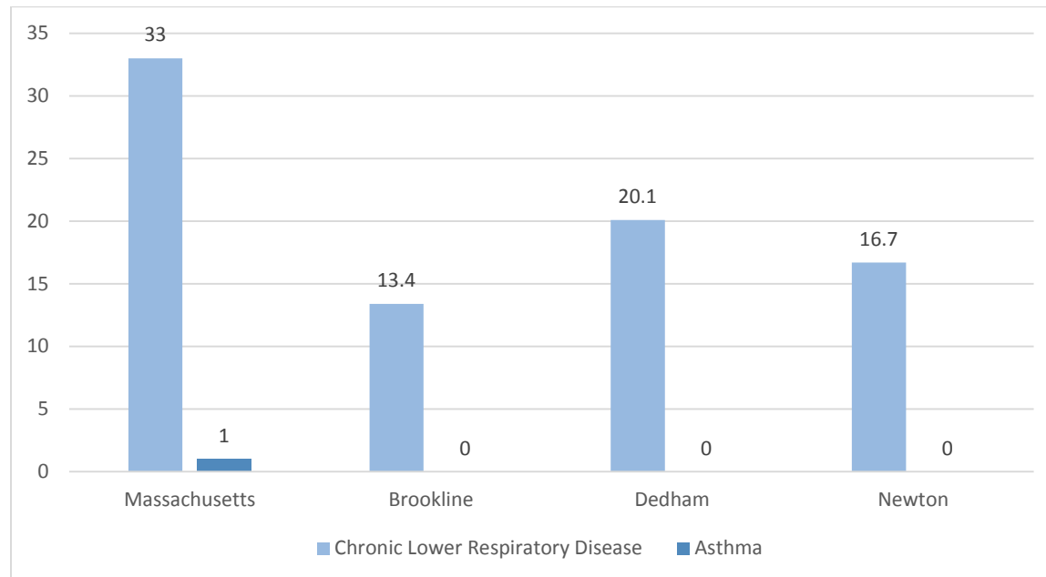
Figure 20: Asthma and Chronic Lower Respiratory Disease Mortality, Age-adjusted Rates per 100,000, 2015
